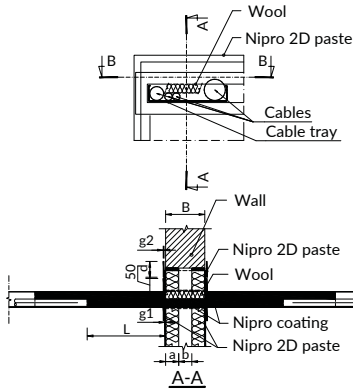
Fig. Protection of cable or cable bundle transitions through a wall made using Niprotec coating and 2D paste.
