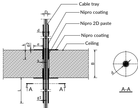
Fig. Protection of single cable or a bundle of cables through ceiling made using Niprotec coating and 2D paste.
